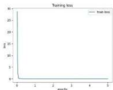
Figure 2: Training Loss
