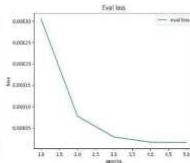
Figure 3: Validation Loss
